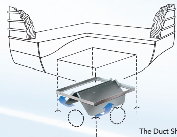
The Duct Shutter in the open position
